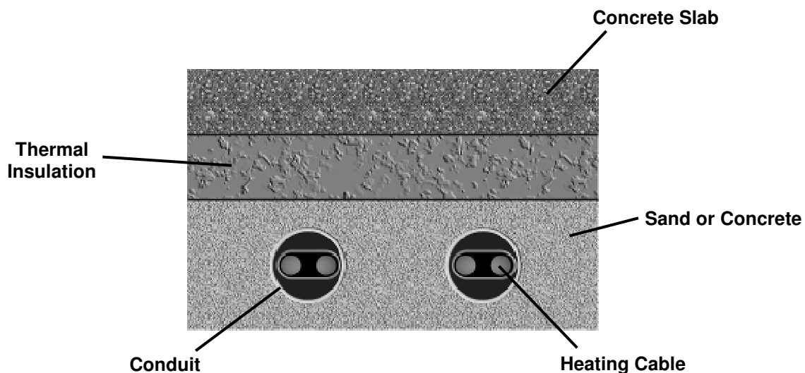
Typical Frost Heave Prevention Sub-Structure
