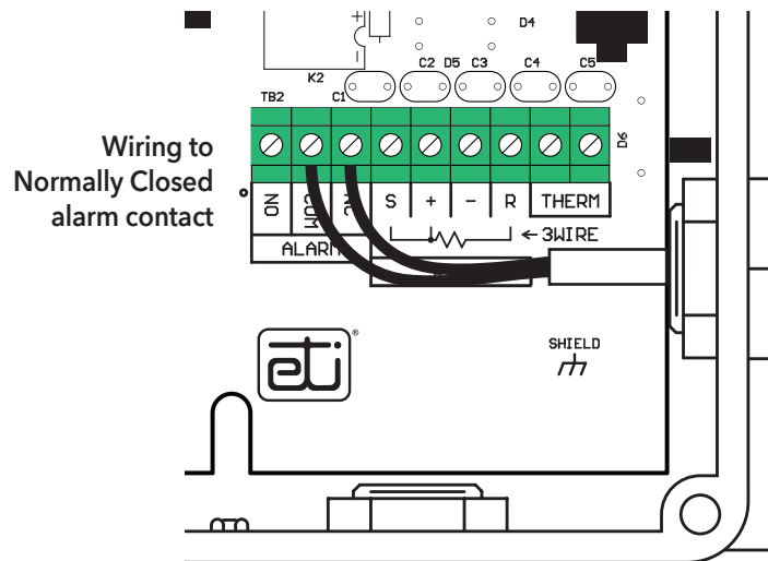
FIGURE 5. External alarm connection
