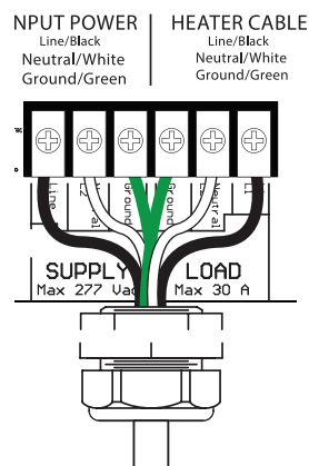
FIGURE 3. Contractor connections.
