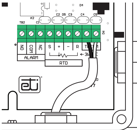
FIGURE 4. Thermistor sensor connection
